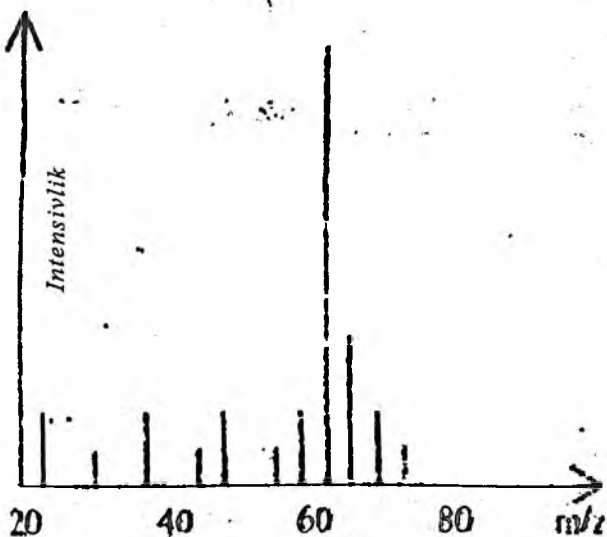
5.15-rasm. Bombardimon molekularlar
