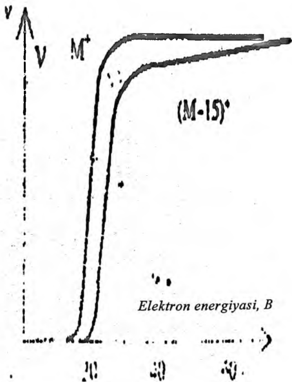
5.14 – rasm. Atseton molekulari
