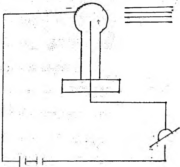
1.6-rasm. Tashqi fotoeffektli fotoelement: 1 – fotokatod; 2 – fotoanod; 3 – shisha lampa; 4 – ko'rsatkich asbob; 5 – tok manbai
