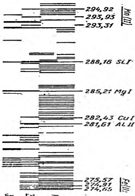
2.10-rasm. Qotishmaning spektri:
