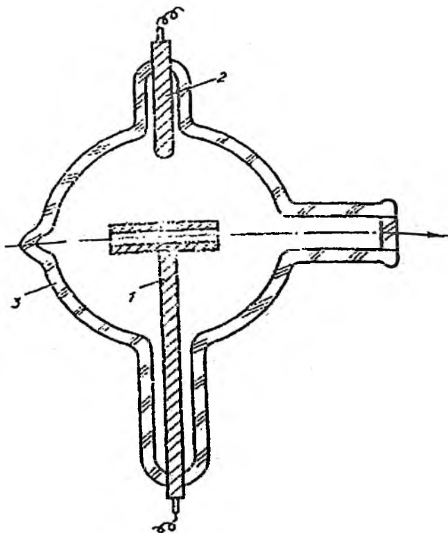
2.6-rasm. Adsorbtsion analizda ishlatiladigan kovak katodli lampa: 1 – katod; 2 – anod; 3 – uchqunlatish nayi.
