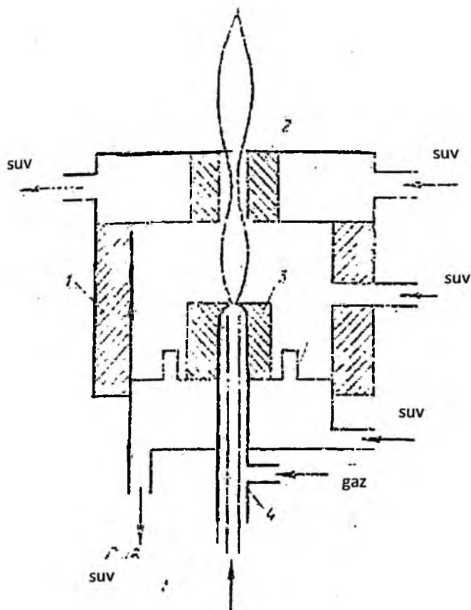
2.3-rasm. Yoy plazmatroni sxemasi: 1-kamera; 2, 3-grafit elektrodlar; 4-purkagich.
