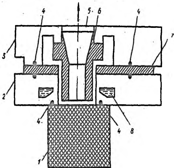
2.7-rasm. Tutovchi razryadli naycha sxemasi:
