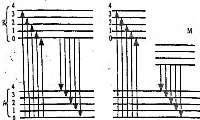
5.10-rasm. Lyuminetsent shulalanish yuzaga kelishining soddalashtirilgan sxemasi
