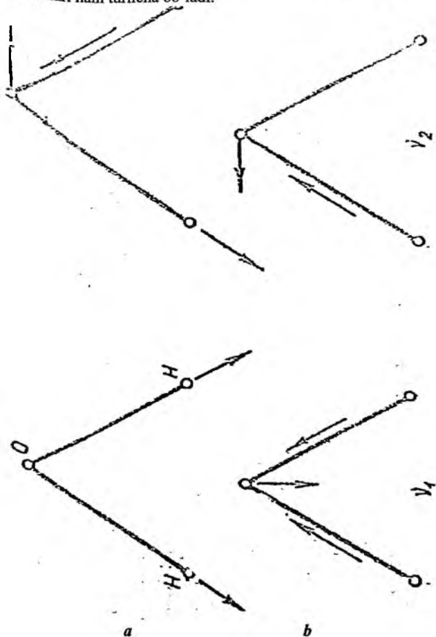
4.1-rasm. H_2O molekulari normal tebranish shakllari
