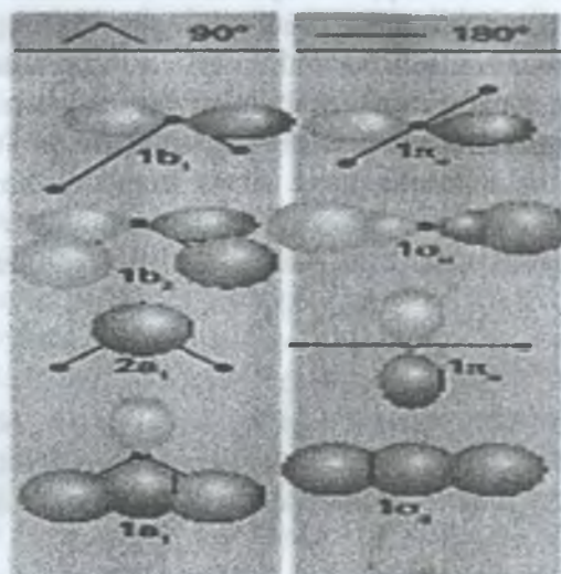
2.28-rasm. XH_2 ning 2.35- rasmida ko'rsatilgan ikki holati molekulyar orbitallari diagrammalari nisbati
