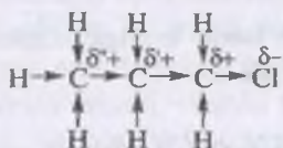
Cl-atomining -I ta'siri
