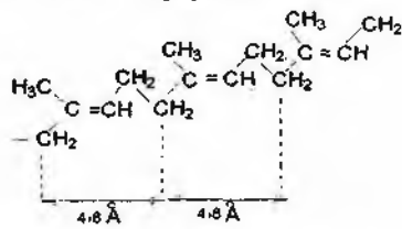
Trans-izomer (guttapercha)
