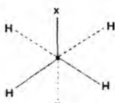
trans -
