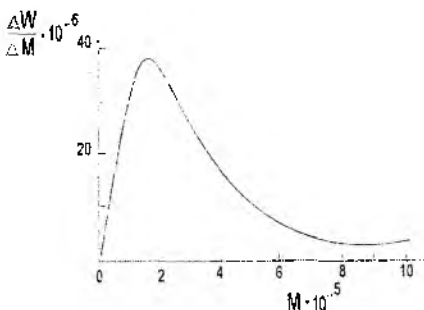
62-rasm. Polimerning molekulyar massa bo'yicha taqsimlanish differensial egrisi.
