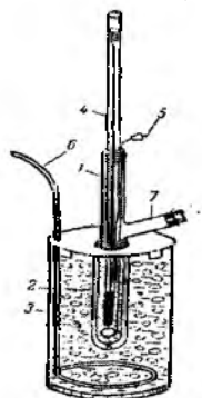
69-rasm. Polimerlar molekulyar massasini krioskopik usulda topish uchun asbob: 1-yon shobchali krioskopik yacheyka; 2-probirka; 3-stakan; 4,6-aralastirgichlar; 5-Bekman termometri; 7-yutuvchi.
