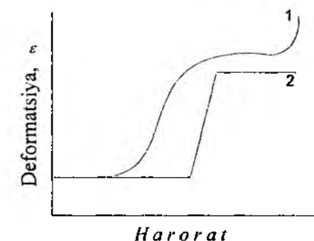
88-rasm. Polimerlarning termomechanik egri chiziqlari; 1 – amorf polimer; 2 – kristall polimer.
