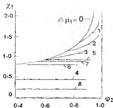
53-rasm. \chi_1 parametrining polimerning eritmadagi hajmiy ulushiga bog'liqligi: 1-tabiiy kauchuk – atseton; 2-tabiiy kauchuk – metiletiketone; 3-tabiiy kauchuk – etilatsetat; 4-tabiiy kauchuk – benzol; 5-polistirol – atseton; 6-polistirol – n-propilatsetat; 7-poliizobutilen – benzol; 8-poliizobutilen – xloroform.
