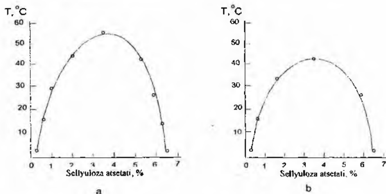
43-rasm. Holat diagrammalari: a – sellyuloza atsetati – xloroform; b – sellyuloza atsetati – dixlorethan
