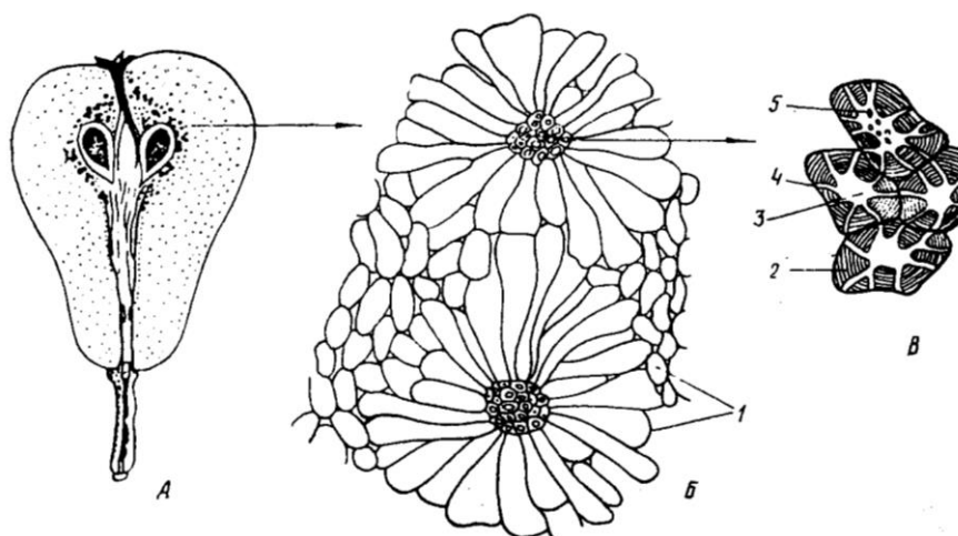
11-rasm. Nok mevasining sklereidlari ( Pyrus communis ):
