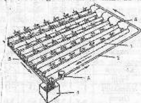
41-rasm. Oqaligan kichik hajmli gidroponika moslama tizimi (Tarakov G.I., 1982)
