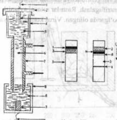
Ilova, 12-rasm. Poliakrilamid gelida preparativ elektroforez aziladigan priboriing sxemasi (A) va unda virus tozalash (B)
