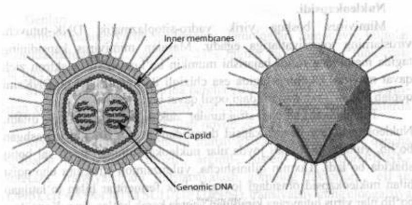
65-rasm. Mimiviruslarning tuzilishi (120)
