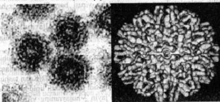
38-rasm. Alfavirusni tashqi ko'rinishi (chapda – mikroskopda olingan rasm, o'ngda – tashqi ko'rinishi) (86)
