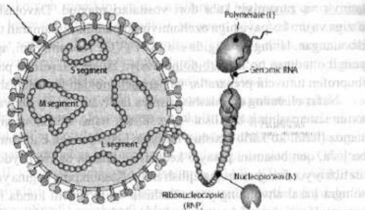
53-rasm. Bunyavirus virionining tuzilishi. Diametri 80 - 120 nm. (104)
