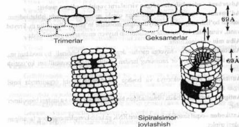
Ilova,22-rasm. TMV oqsilini polimerizatsiya jarayonining sxematik ko'rinishi
