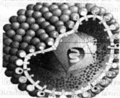
26-rasm. Herpes virusining tuzilishi (71)
