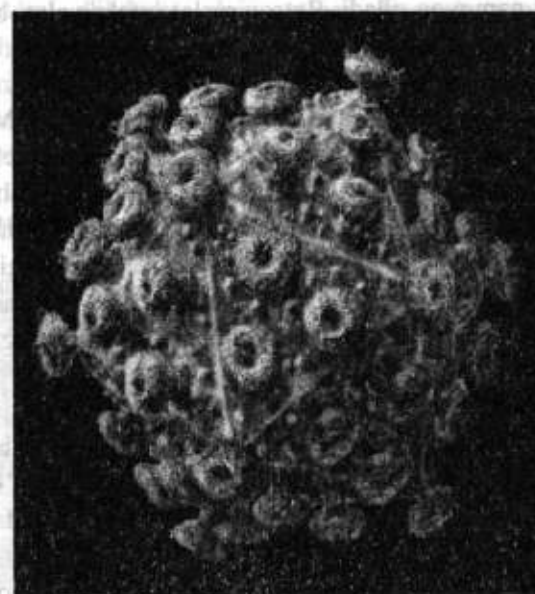
59-rasm. VICH virionining (chapda) tuzilishi, (o'ngda) tashqi ko'rinishi (112) m
