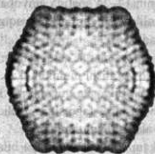
68-rasm. Virofagning sputnigi (122)
