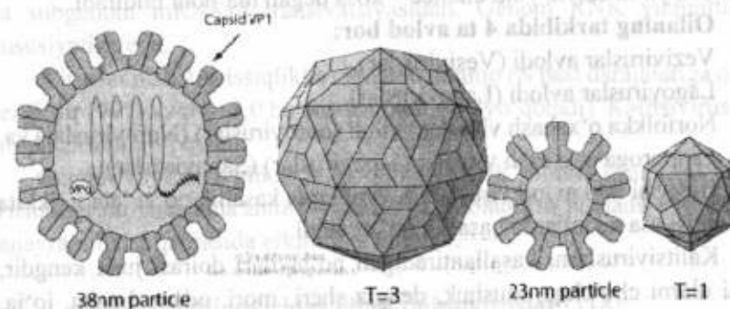
62-rasm. Kalitsiviruslar virioni
