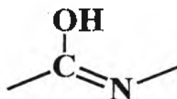
Enol - shakli
