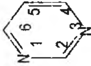
Pyrimidin
