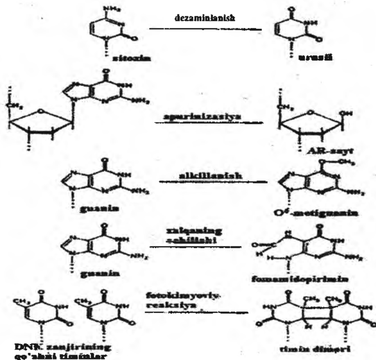
26- rasm. DNK jarohatlanishining ba'zi turlari
