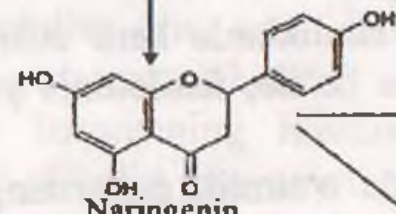
Naringenin (flavonon)
