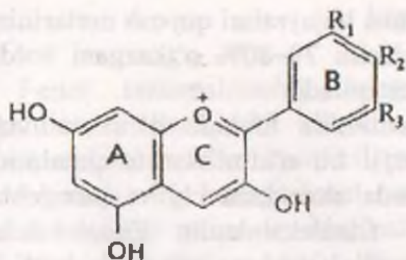
Antostionidin
