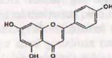
Apigenin (flavon)
