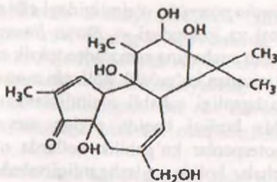
Forbol
