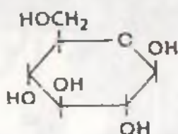
\beta -D-glyukoza
