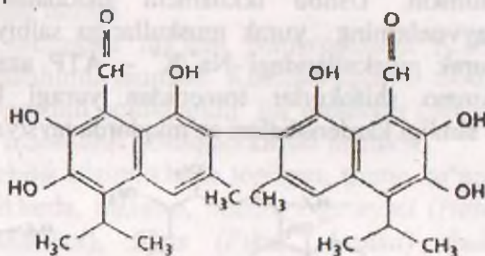
Gossipol
