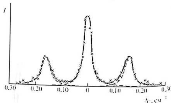
4.22 rasm. Majburiy kombinatsion sochilishning spektri.
