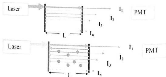
6.11 rasm. Rezonator ichida moddalarning yutilish koeffitsientini aniqlash usuli. a) bo'sh rezonator, b) gaz solingan rezonator.
