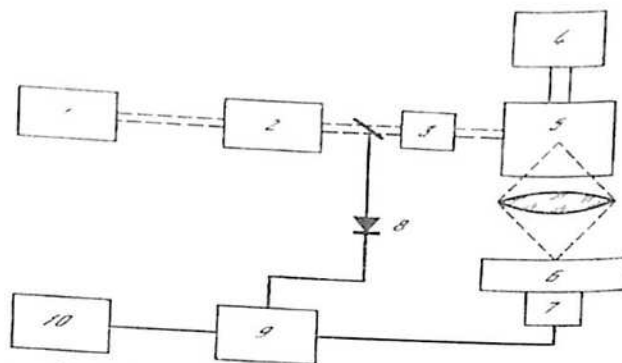
6.1 rasm. Lazerli atom- fluorescent spektrometrning blok-sxemasini: 1- lazer, 2- bo'yoq lazeri, 3- optik sistema, 4- elektr ta'minoti bloki, 5- atomizator, 6- spektral filtr, 7-fotokuchaytirgich, 8-fotodiod, 9-strob integrator, 10-samopisets.
