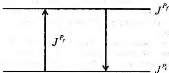
4.9-rasm. Yadroda radiatsion o'tishlar.
