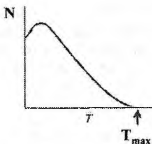
4.4-rasm. Beta-parchalanish spektri.
