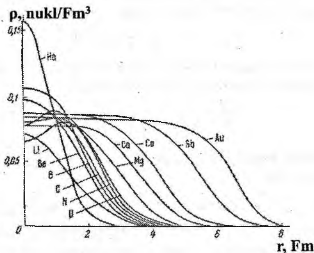
1.6-rasm. Atom yadrosida zaryad taqsimoti.
