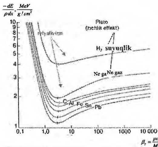
6.1-rasm Ionizatsion yo‘qotish.
