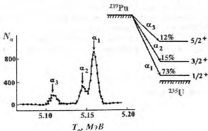
4.3 - rasm. Plutoniy ^{239}\text{Pu} yadrosining \alpha -parchalanish sxemasi.
