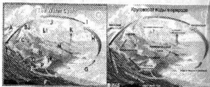
9.1-rasm. Tabiatda suvning aylanishi
