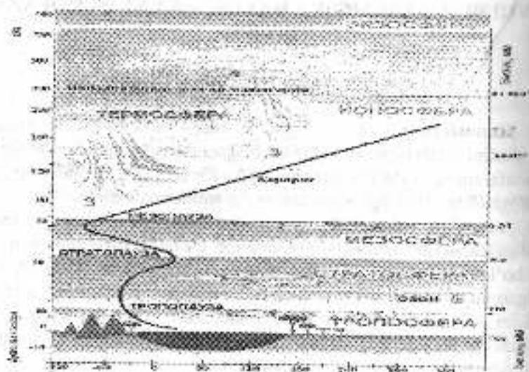
8.1-rasm. Atmosferaning vertikal tuzilishi (R. Ramade, 1998 y)
