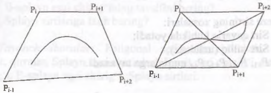
2.13-rasm. B-splayn egri chizig'i.
