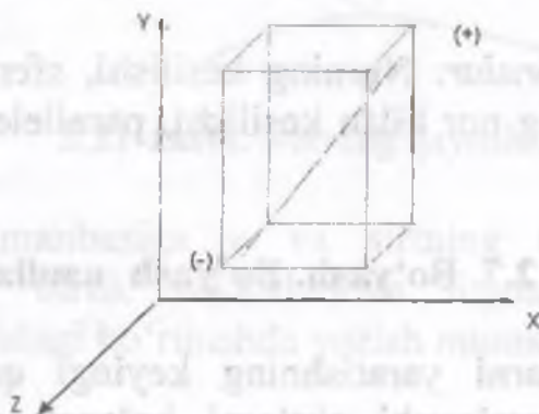
2.20-rasm. Parallelepiped.
