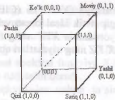
2.29-rasm. RGB rangli kub.
