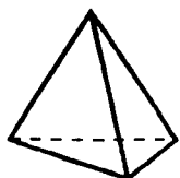
Tetraedr
