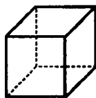
kub
