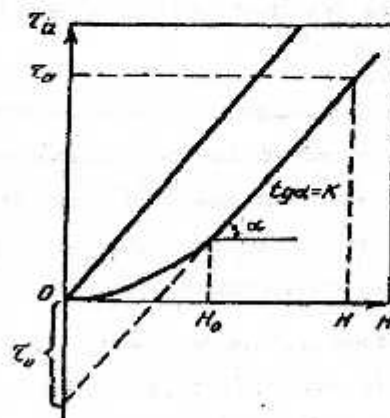
4.20-rasm. Qatlamning adsorbsion himoya qilish vaqti \tau_a ning adsorbent qatlami balandligi H dan bog'liqligi
