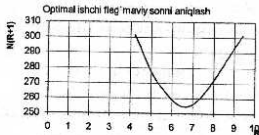
4.17-rasm. Bog'liqlik N(R+1) dan R gacha.
