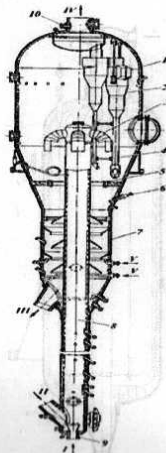
32-rasm. Changsimon katalizatorli reaktor:
