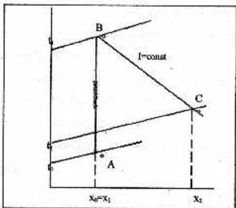
4.2-rasm. Nazariy quritish jarayonining I-x diagrammasida tasvirlash.
