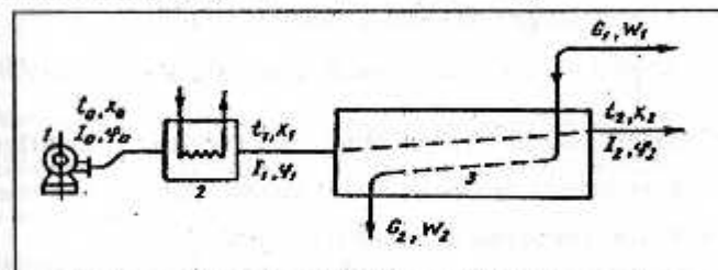
4.1-rasm. Normal quritish jarayonining sxemasi:
