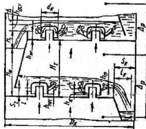
4.12-rasm. Qalpoqchali tarelkalar qarshiligini hisoblash
