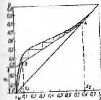
4.19-rasm. Relativatsion kolonna tarelkalarining sonini grafik usulda aniqlash.
