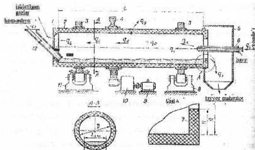
4.4-rasm. Aylanuvchan barabanli o'txona:
