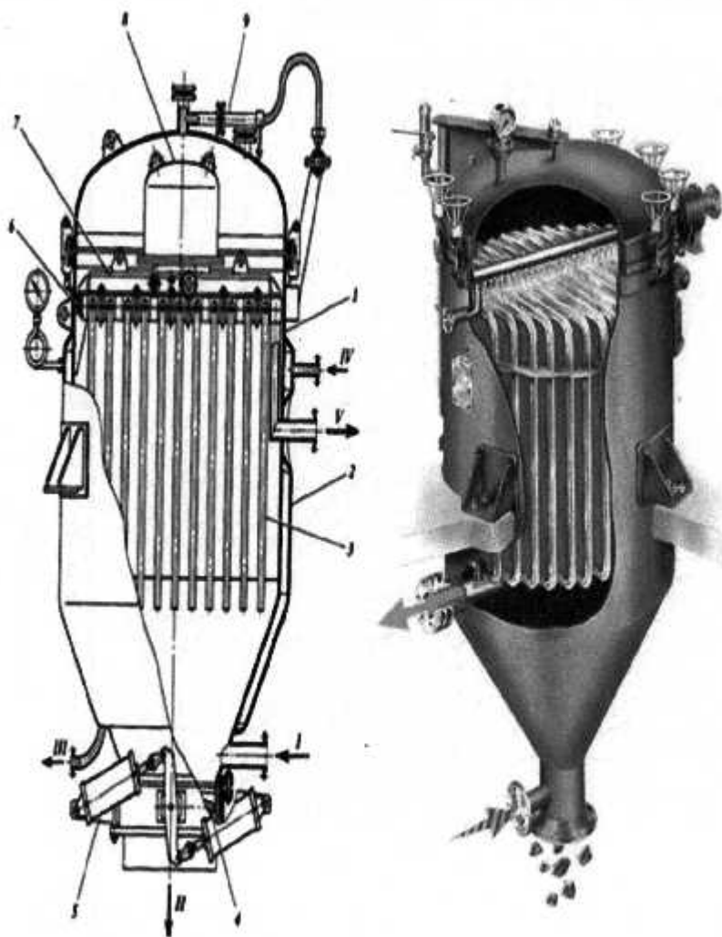
10-rasm. Listli filtr tuzilishi:
