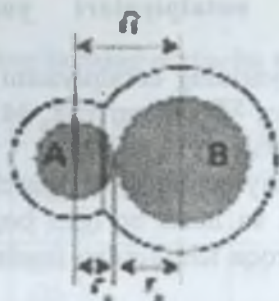
18 Covalent radius
