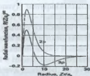
1.8-rasm. Vodorodsimon atomning 2p va 3p orbital-larining radial taqsimlanish grafigi
