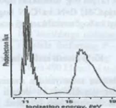
2.19-rasm. \text{NH}_3 ning UB sohadagi He 21eV nurlanishi yordamida olingan fotoelektron spektri
