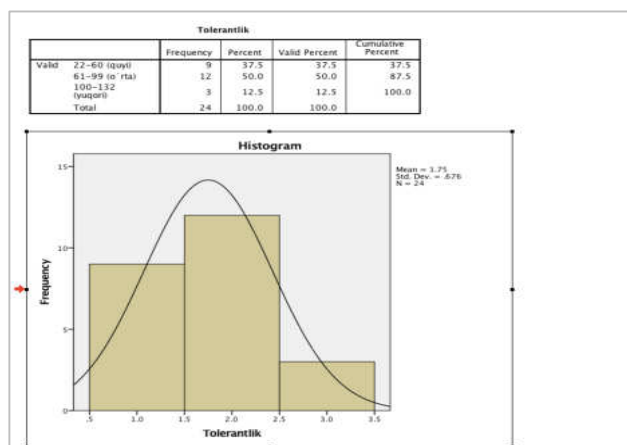
18.27. Rasm. Gistogrammaning normal taqsimotga mosligi.
