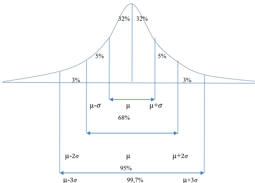
3.1-rasm. Normal taqsimlanish modeli.
