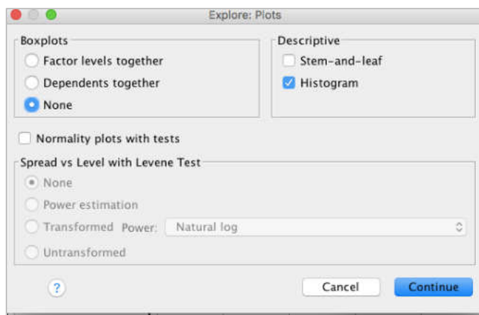
18.28. Rasm. Gistogramma qurish uchun Explore dialog oynasini ochish.
