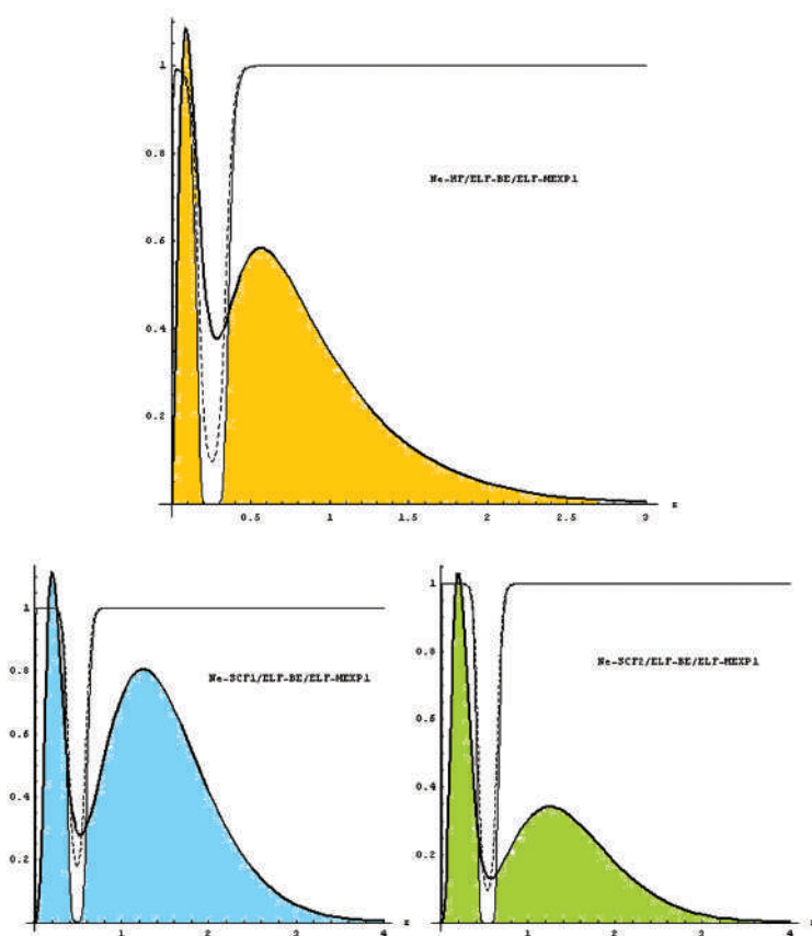
FIGURE 5.8 (Up and down) The comparative rescaled Ne radial density structure (—) given by Eq. (5.436) with the electron localization functions (ELFs) of Becke-Edgecombe BE (---), given in Eq. (5.388), and with the Markovian exponential one MEXP1 (—), given by (5.419), through different levels of self consistent field (SCF) methods: Hartree-Fock (HF) set (5.428)–(5.430), simplified SCF1 as the first orbital approximation set (5.431), (5.432), independently of angular number, and the simplified SCF2 as the second orbital approximation set (5.433)–(5.435), dependently on the angular number, respectively; after Putz (2005).
