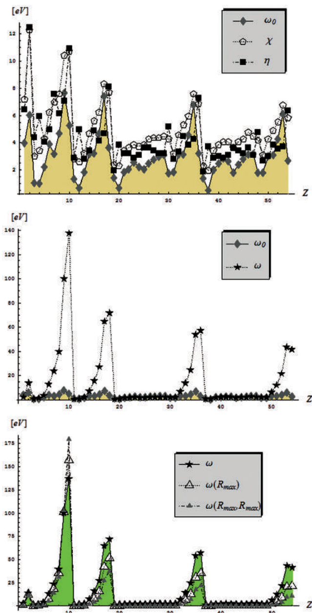
FIGURE 4.18 Atomic scales of reference, actual global, local at R_{\max} and kernel at (R_{\max}, R_{\max}) electrophilicities, as computed by Eqs. (4.234), (4.346), (4.345), and (4.344), respectively, with the values of Table 4.14 (Putz & Chattaraj, 2013).
