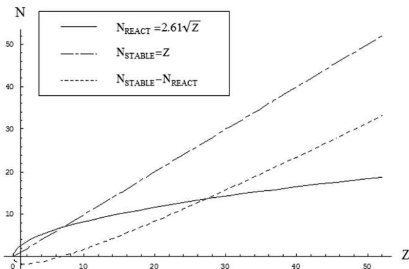
FIGURE 4.6 The comparative shapes of the valence electrons to be engaged in chemical reactivity (continuous curve) computed using Eq. (4.151) based on the combined optimal Bohm total energy (4.148) with the golden ratio imbalance of Eq. (2.9), respecting the stable physical case (dot-dashed curve), and of their differences (dashed curve); all originate at the 0th atom (the neutron, Z=0 ) (Putz, 2012a).
