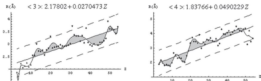
FIGURE 4.22 Global (linear) and local (high order polynomial) regressions plots for atomic radii using Boyd-Markus electronegativity's scale with experimental (left) and basis set pseudopotential (right) Mulliken values; after Putz (2012c).
