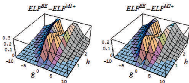
FIGURE 5.5 The same kind of representation as in Figure 5.4, yet here for marking the Markovian (M1+) and (M2+) behaviors of Eqs. (5.419) and (5.420), in left and right, respectively (Putz, 2009).
