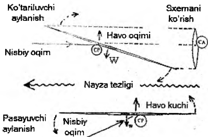
76-rasm. Nayzaning uchish vaqtida "o'zini tutishi"
