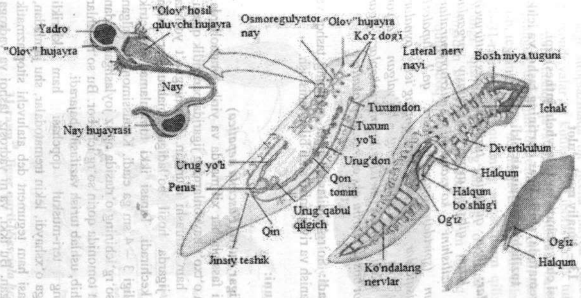
29-rasm 19 . Palanariyaning ichki tuzilishi.
